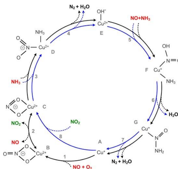
Scheme 1. Possible mechanism of SCR reaction. The fast SCR cycle is shown in blue, the NO activation cycle - in black. Reactants are indicated in red, reaction products - in black, and the \text{NO}_2 intermediate - in green. Reproduced with permission from Janssens et al. [7]. Copyright (2015) American Chemical Society.
