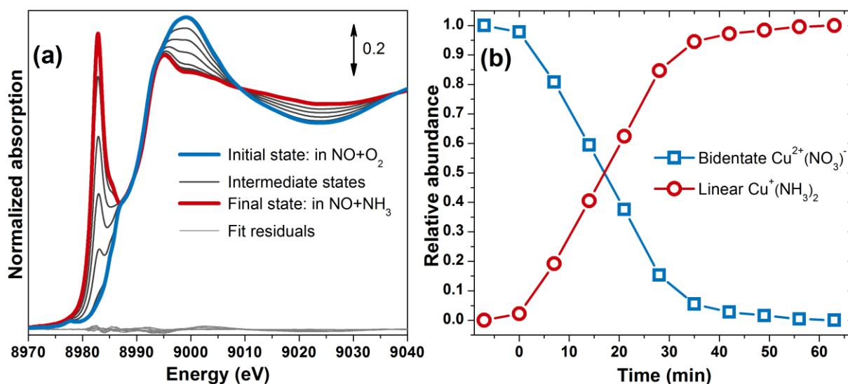
Figure 8. (a) Evolution of Cu K-edge XANES spectra of Cu-SSZ-13 after switching from 1000 ppm NO + 10% \text{O}_2 flux (initial state) to 1000 ppm NO + 1200 ppm \text{NH}_3 flux (intermediate states and final state) at 200 °C (b) Relative abundance of \text{Cu}^{2+}(\text{NO}_3)^- bidentate nitrate and linear \text{Cu}^+(\text{NH}_3)_2 complex after changing the flux composition from \text{NO}+\text{O}_2 to \text{NO}+\text{NH}_3 . The moment when the fluxes were switched and the measurement of the first “intermediate” spectrum was initiated corresponds to time 0. Each pair of points in panel (b) was obtained performing a linear combination fit of the corresponding intermediate spectrum presented in panel (a) considering the spectra of the initial and final states as standards. Unscaled residuals of all fits are presented in the bottom panel (a).
